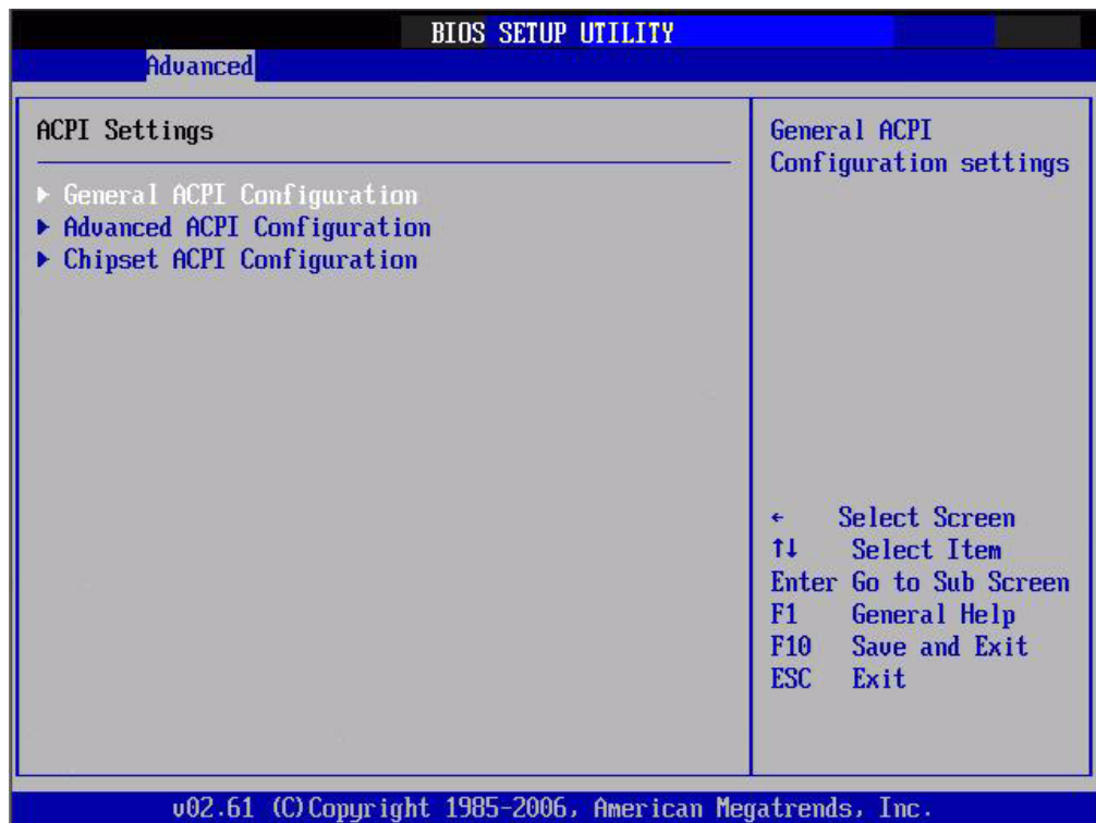
Figure 3.9 ACPI Settings
