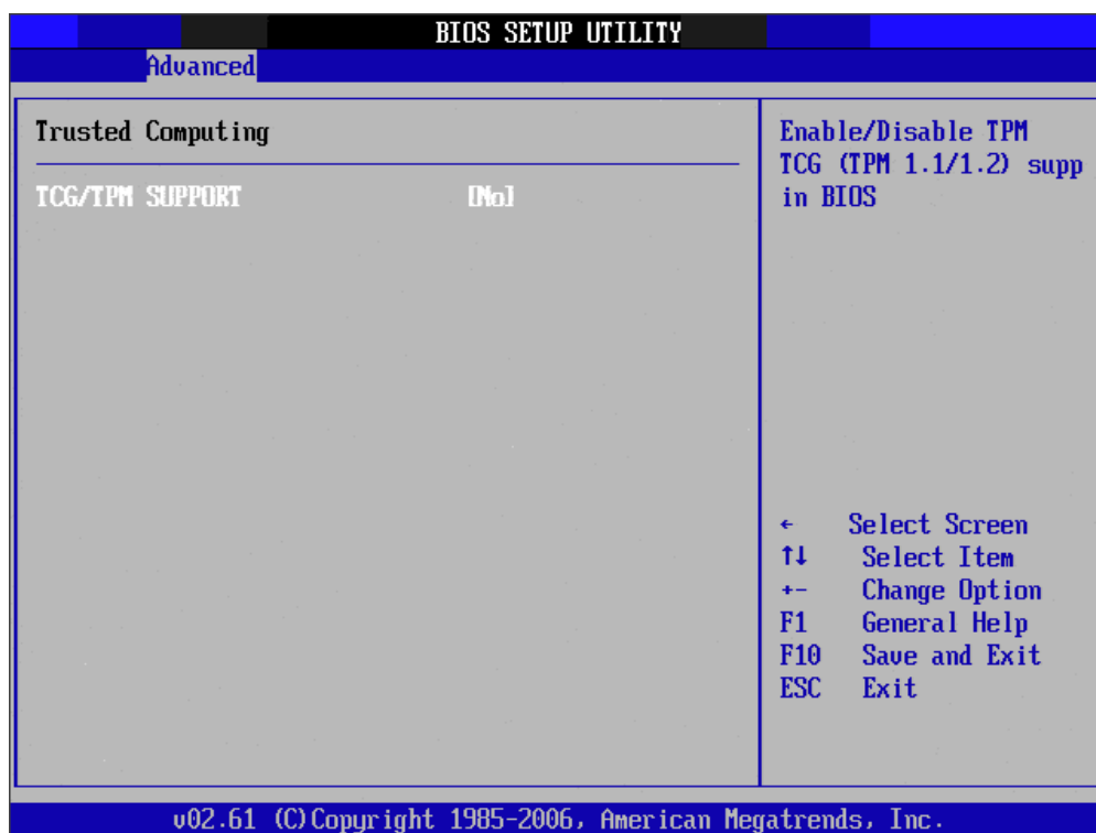
Figure 3.15 Trusted Computing
