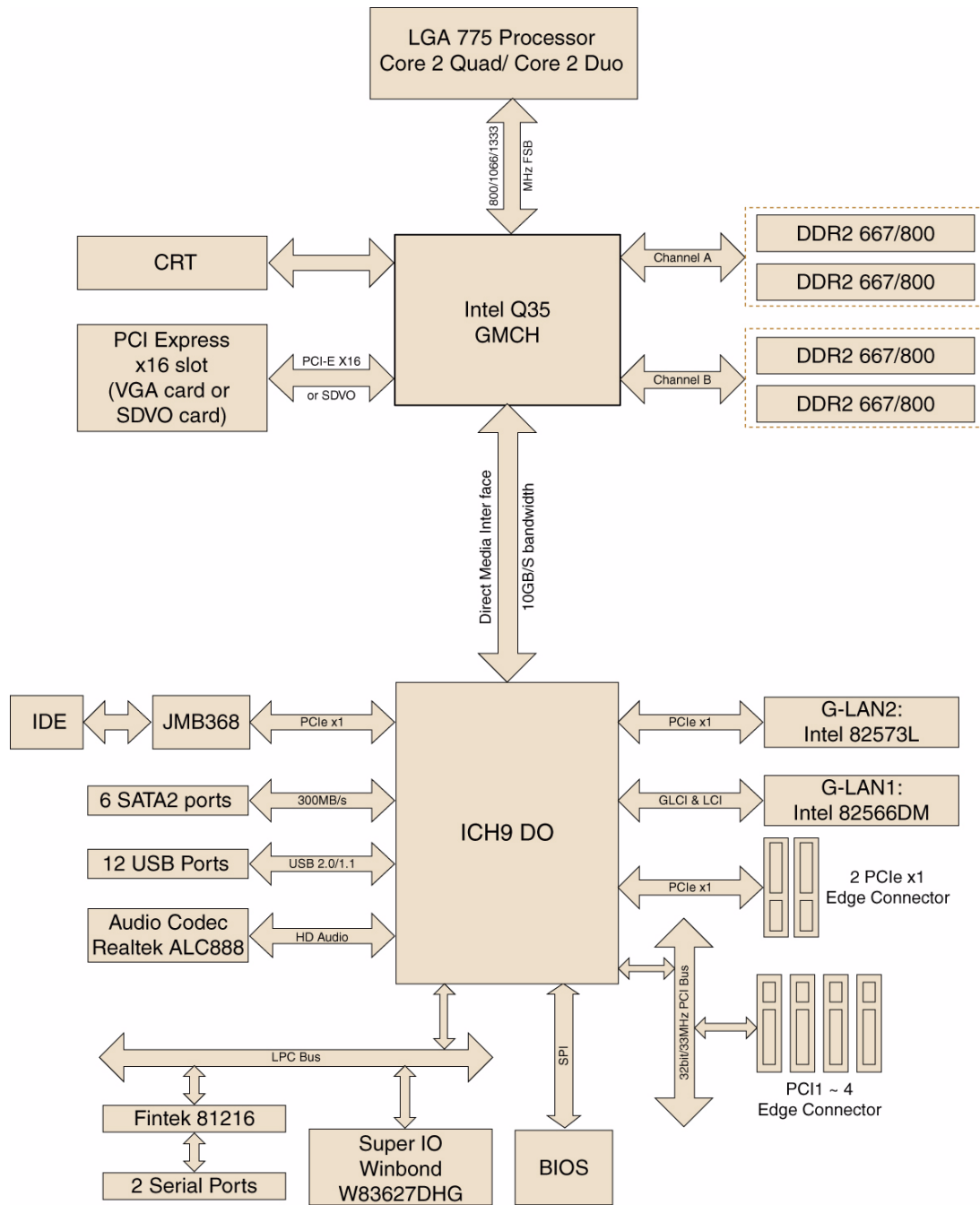
Figure 1.3 AIMB-766 Block Diagram
