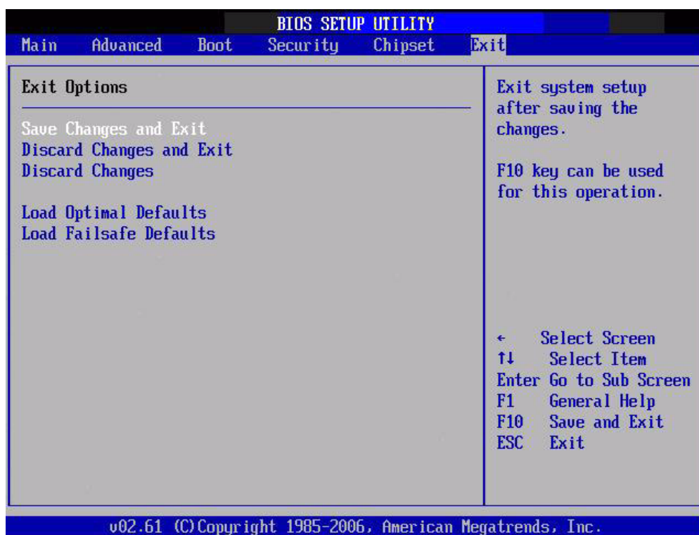
Figure 3.25 Exit Option
