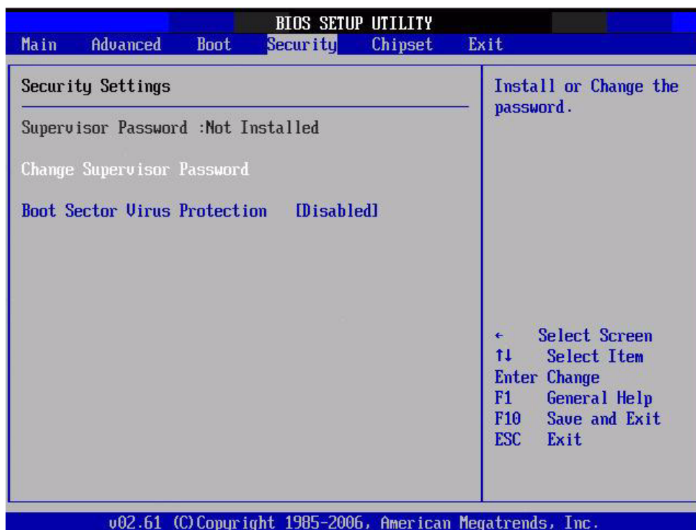
Figure 3.19 Password Configuration
