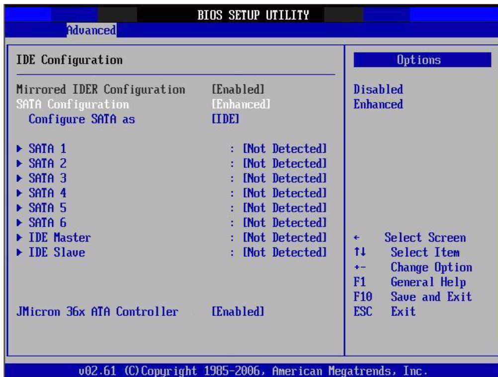
Figure 3.6 IDE Configuration
